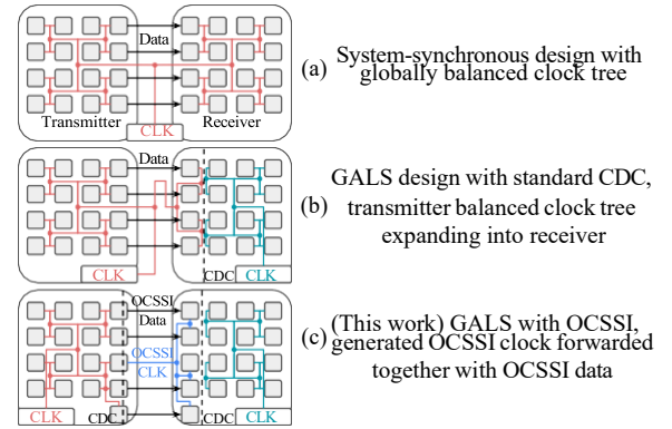
Fig. 3. Different SoC clock distribution methodologies. GALS with OCSSI makes large-scale SoC integration fast, flexible and verifiable with minimized dependencies between Intellectual Property (IP) blocks.
